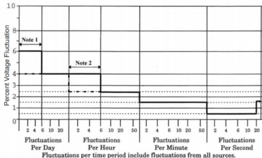
Figure 7.1 – TCLP Flicker Allowances (non-self induced)
